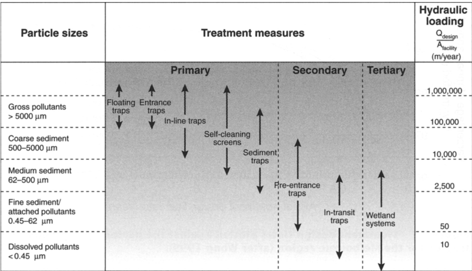
Figure 7.2 Desirable design ranges for treatment measures and pollutant sizes (adapted from Wong 1999).
