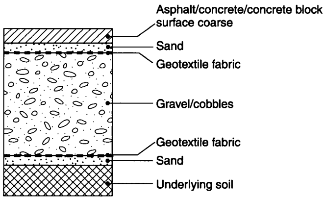
Figure 7.26 Porous pavements.
