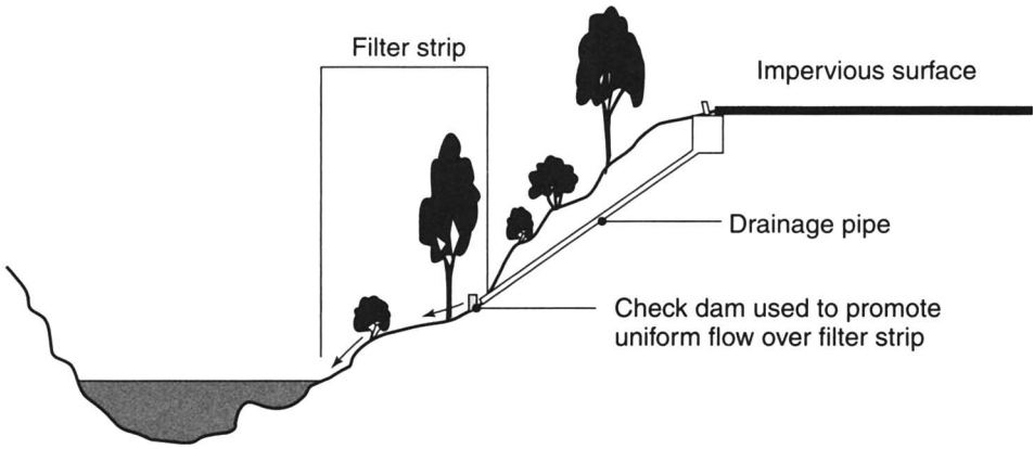
Figure 7.45 Section illustration of kerb and channel and filter strip run-off management option.
