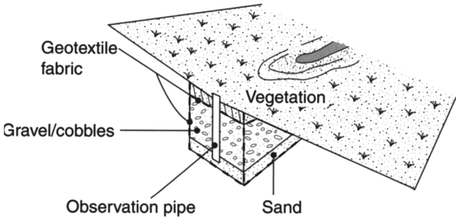
Figure 7.27 Infiltration trench.
