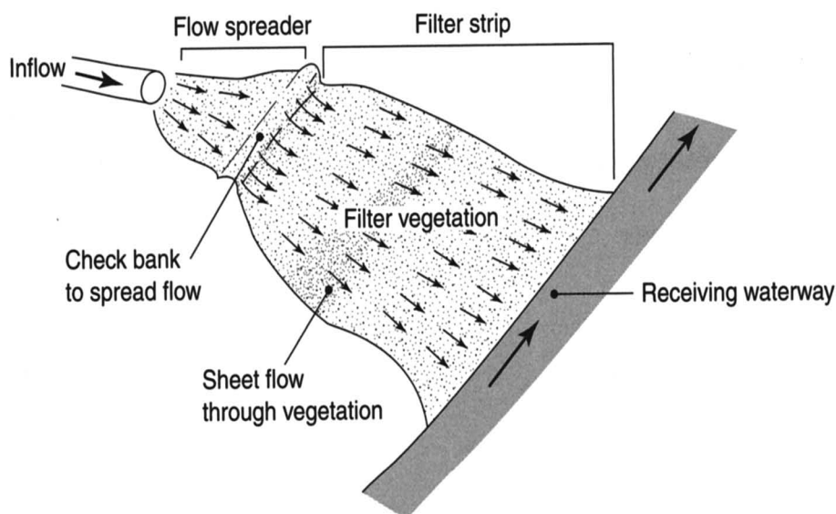
Figure 7.23 Filter strips.
