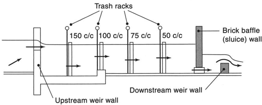
(b) Section through the screens
