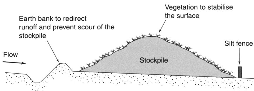
Figure 6.12 Stockpile management.
