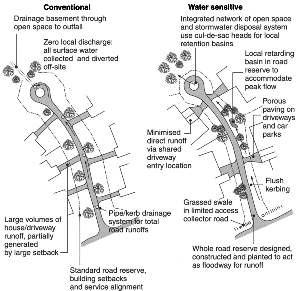
Figure 5.8 Cul-de-sac streetscapes.
