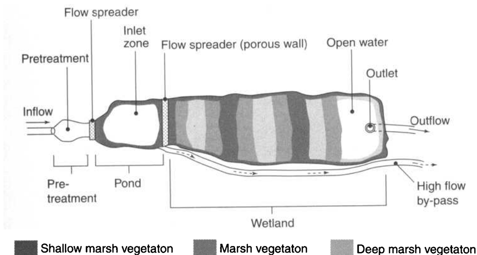
Figure 7.32 Schematic representation of a constructed wetland system.
