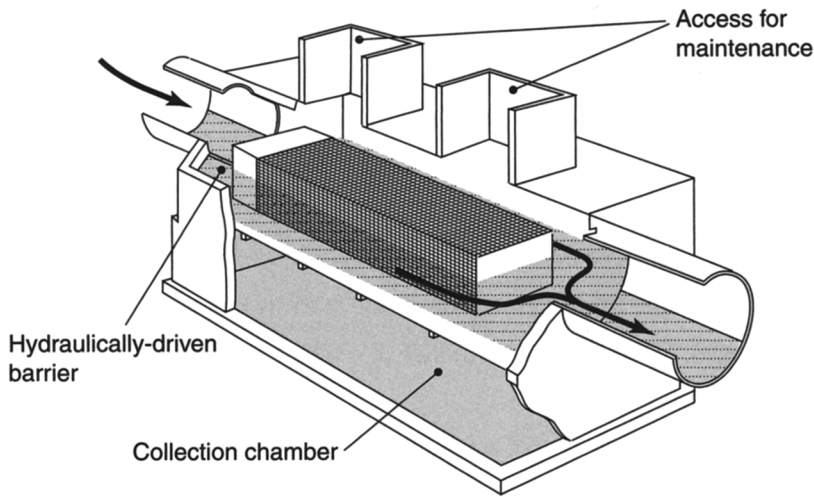
Figure 7.14 Return flow litter baskets (after Ecosol 1997).
